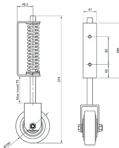
Side Elevation
